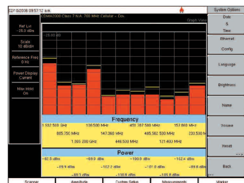
Concentrate on the Signals of Interest
