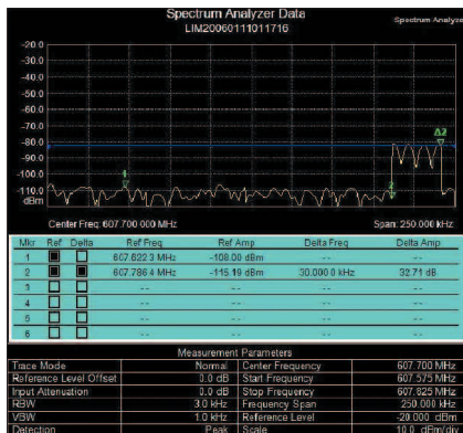
A Discrete Interfering Signal
