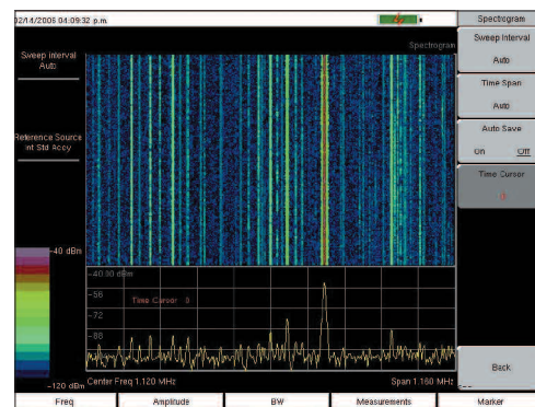
See What is Happening in the Spectrum of Interest
